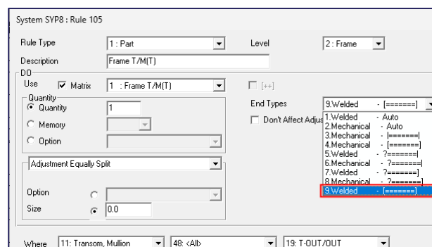
End Type for 90° Welded Joints
