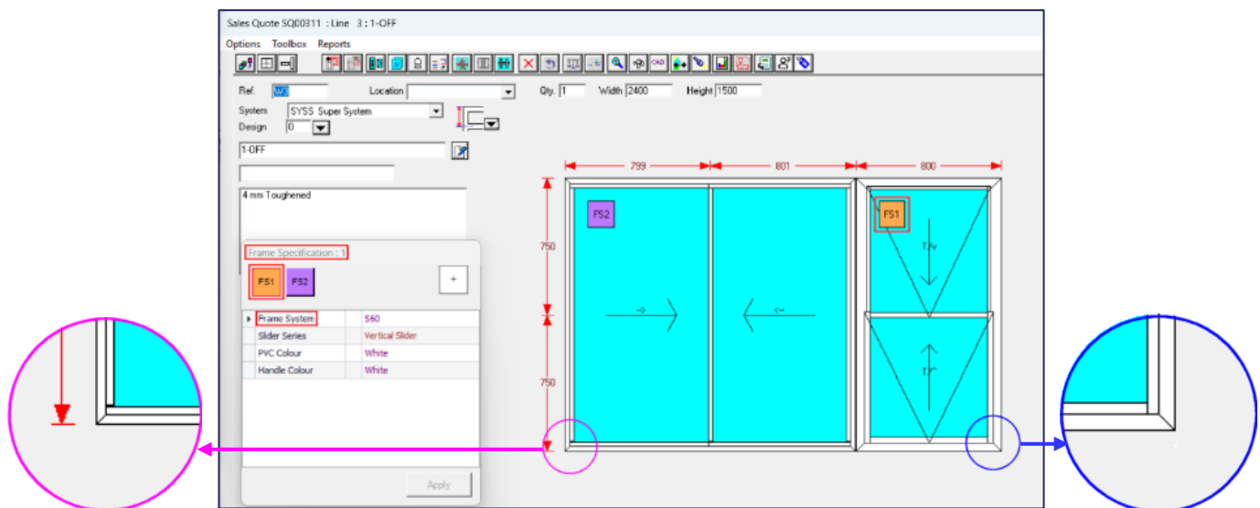
Horizontal Full Length Sash Join
