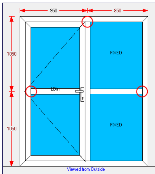
90° Transom/Mullion Welded joints
